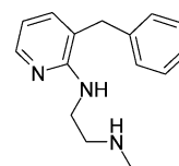
Figure 2. Structure of the side-product formed in the synthesis of ( S )-mirtazapine.
