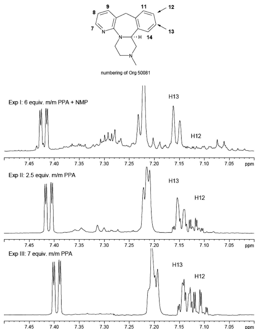
Figure 3. ^1\text{H} NMR spectra (600 MHz in acetone) obtained after the ring-closure step under different reaction conditions.
