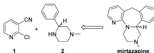
Scheme 1. Retrosynthesis of mirtazapine.
