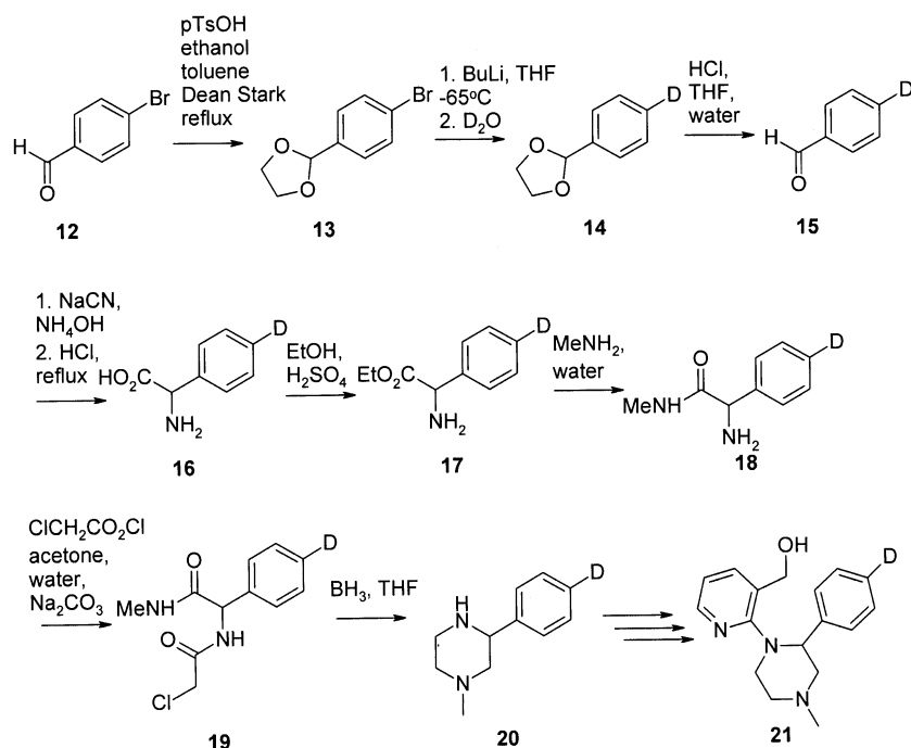
Scheme 4. Synthesis of p -deuteriophenyl alcohol 21 .
