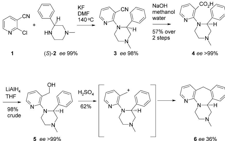
Scheme 2. Synthesis of ( S )-mirtazapine.
