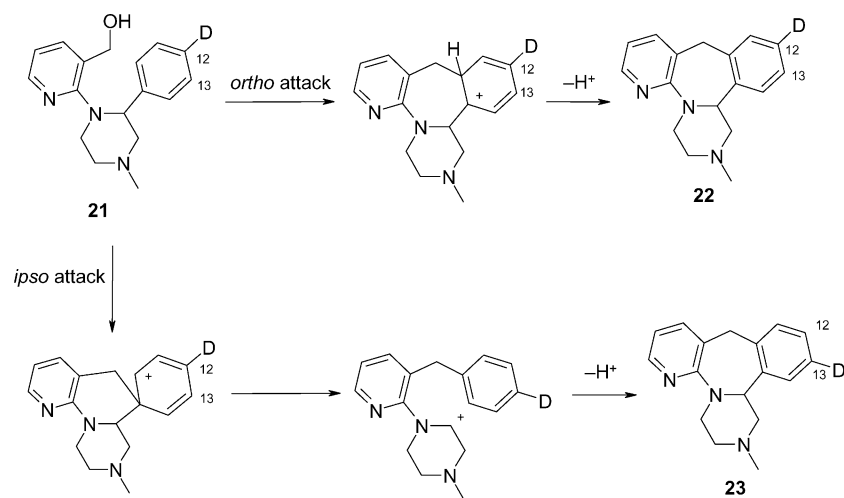
Scheme 5. Anticipated position of the deuterium atom in mirtazapine after ortho and ipso attack.
