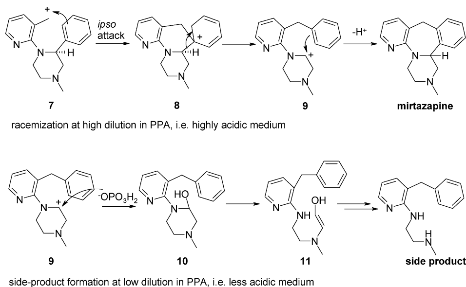
Scheme 3. Mechanism proposed for the racemization and side-product formation.
